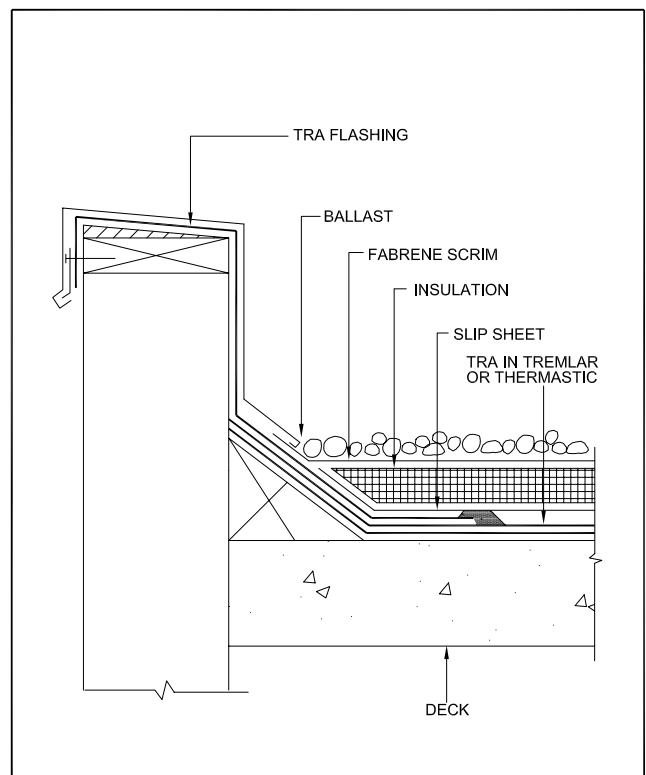
TRA-504 Parapet Wall Flashing Detail
