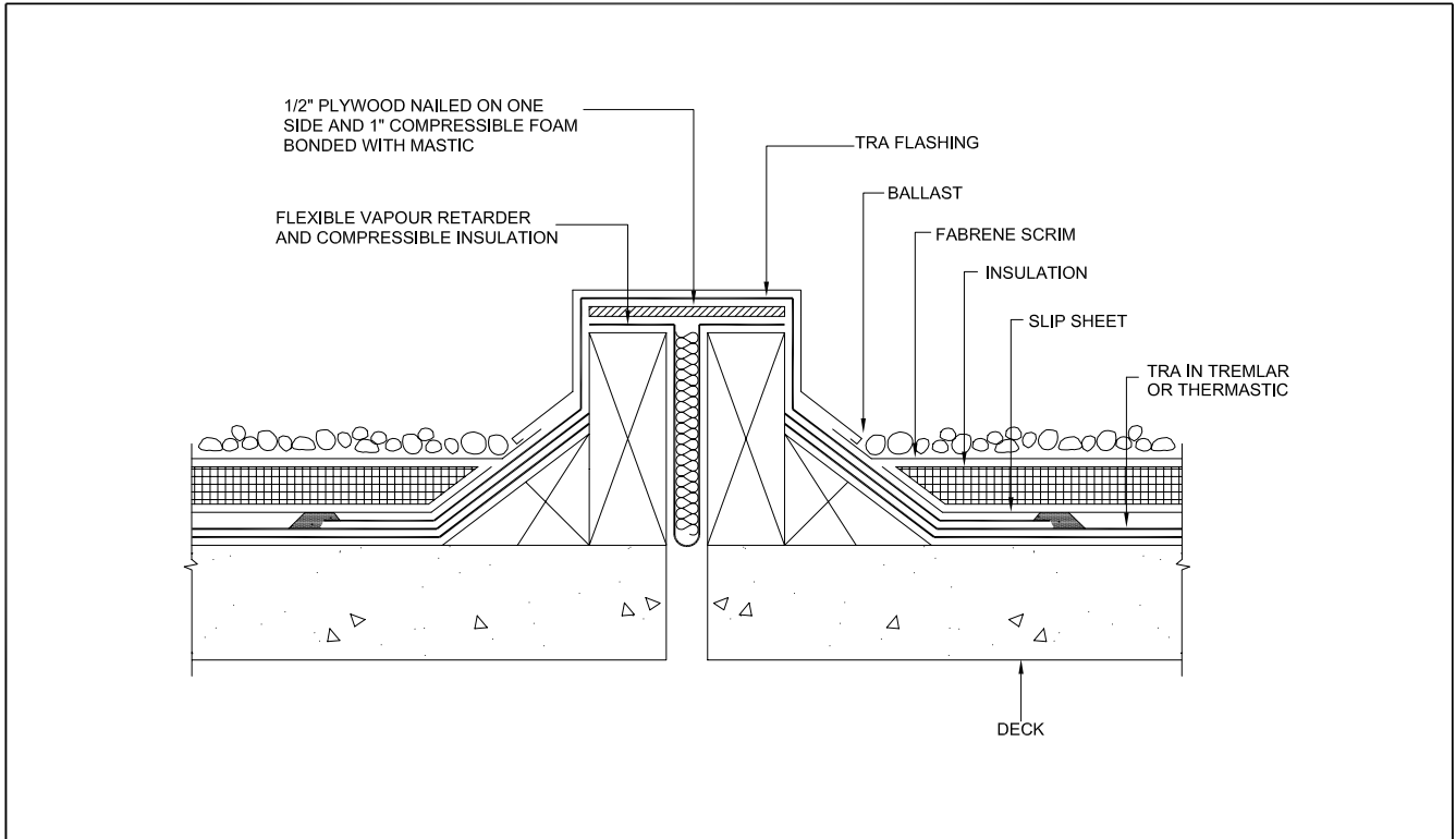
TRA-505 Expansion Joint Flashing Detail
