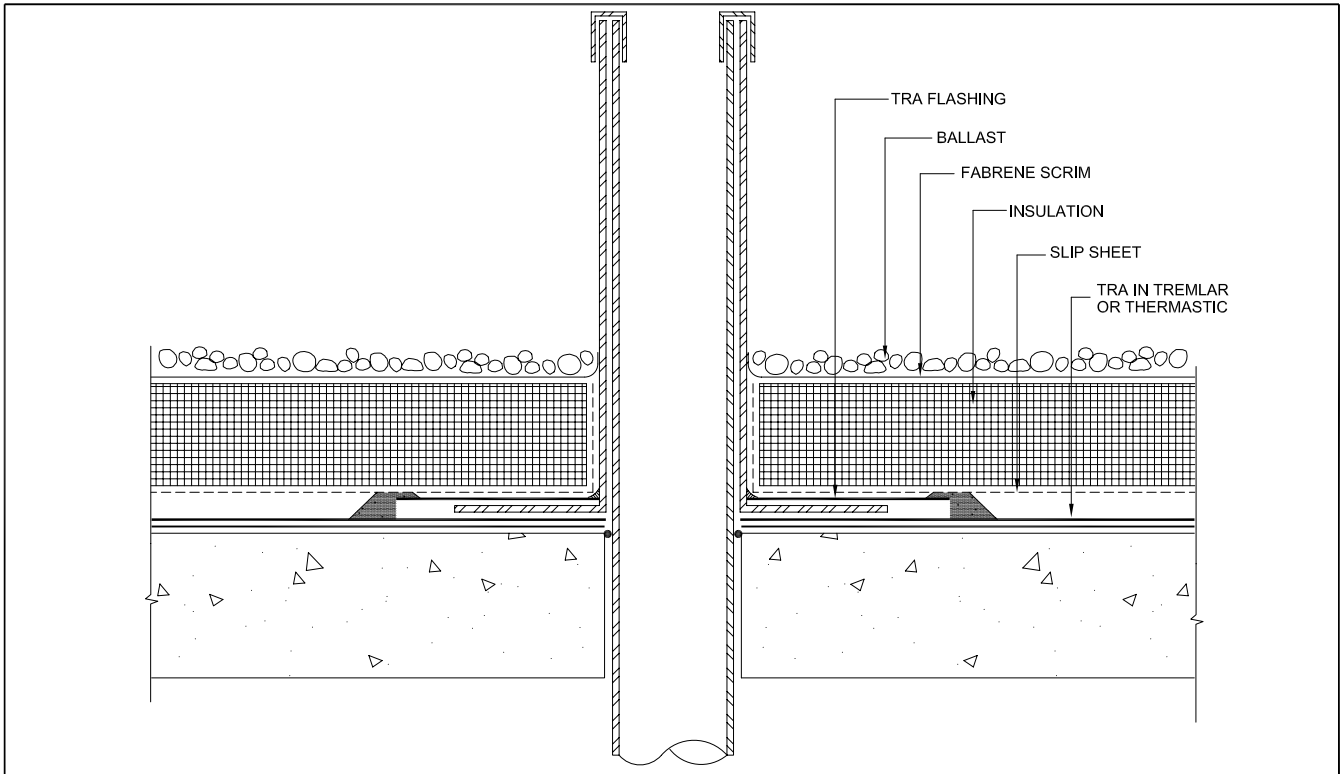
TRA-507 Projection Flashing Detail
