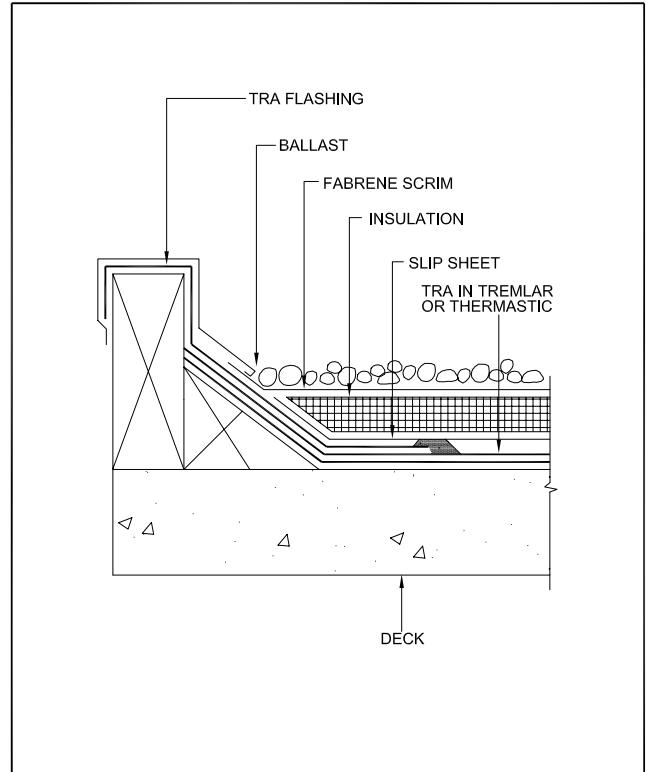
TRA-502 Curb Flashing Detail
