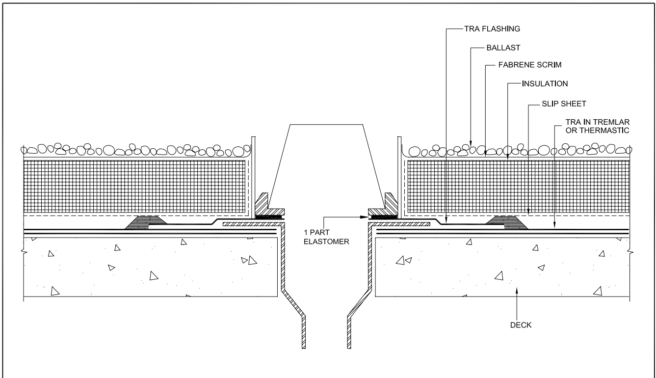
TRA-506 Drain Flashing Detail
