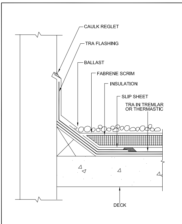
TRA-503 Wall Reglet Joint Flashing Detail
