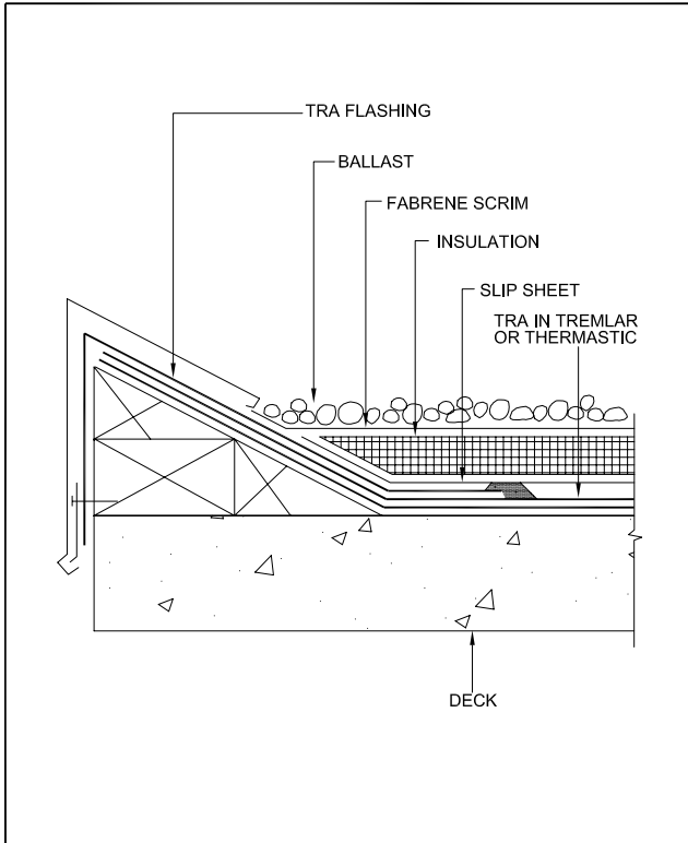
TRA-501 Canted Eave Flashing Detail
