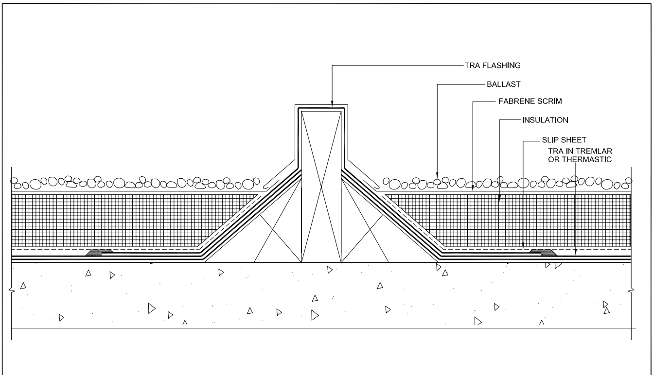
TRA-508 Sleeper Flashing Detail
