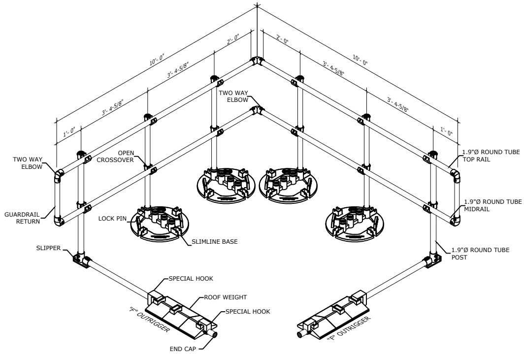
ISOMETRIC
