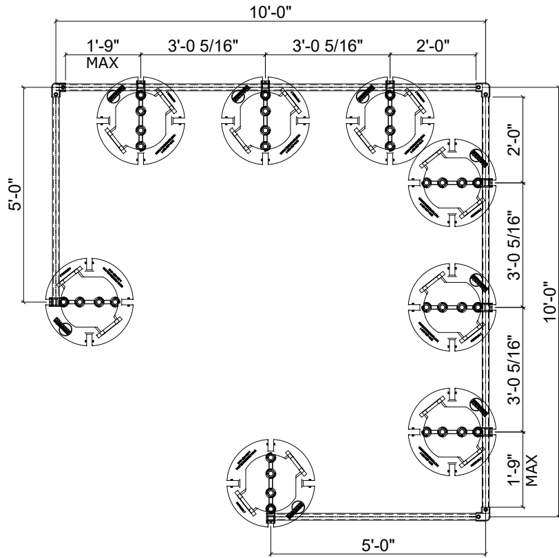
PLAN VIEW
