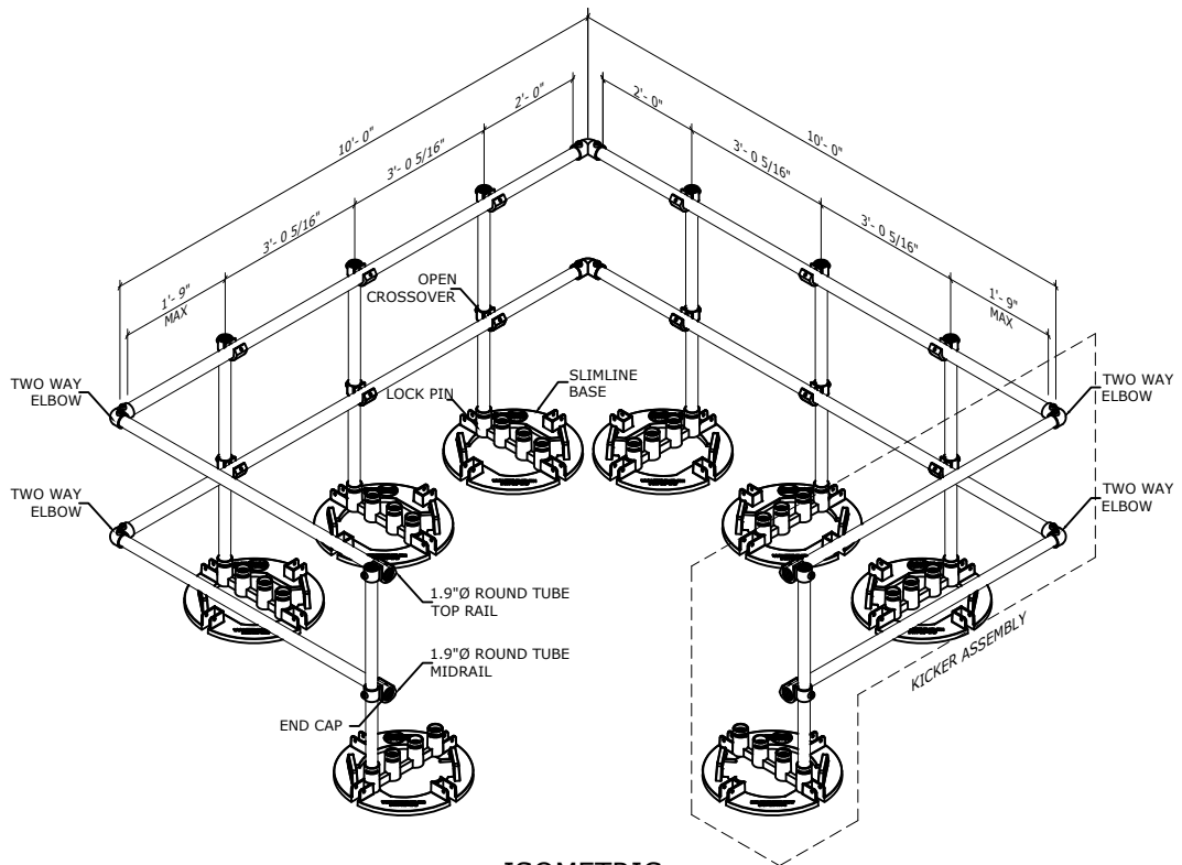
ISOMETRIC
