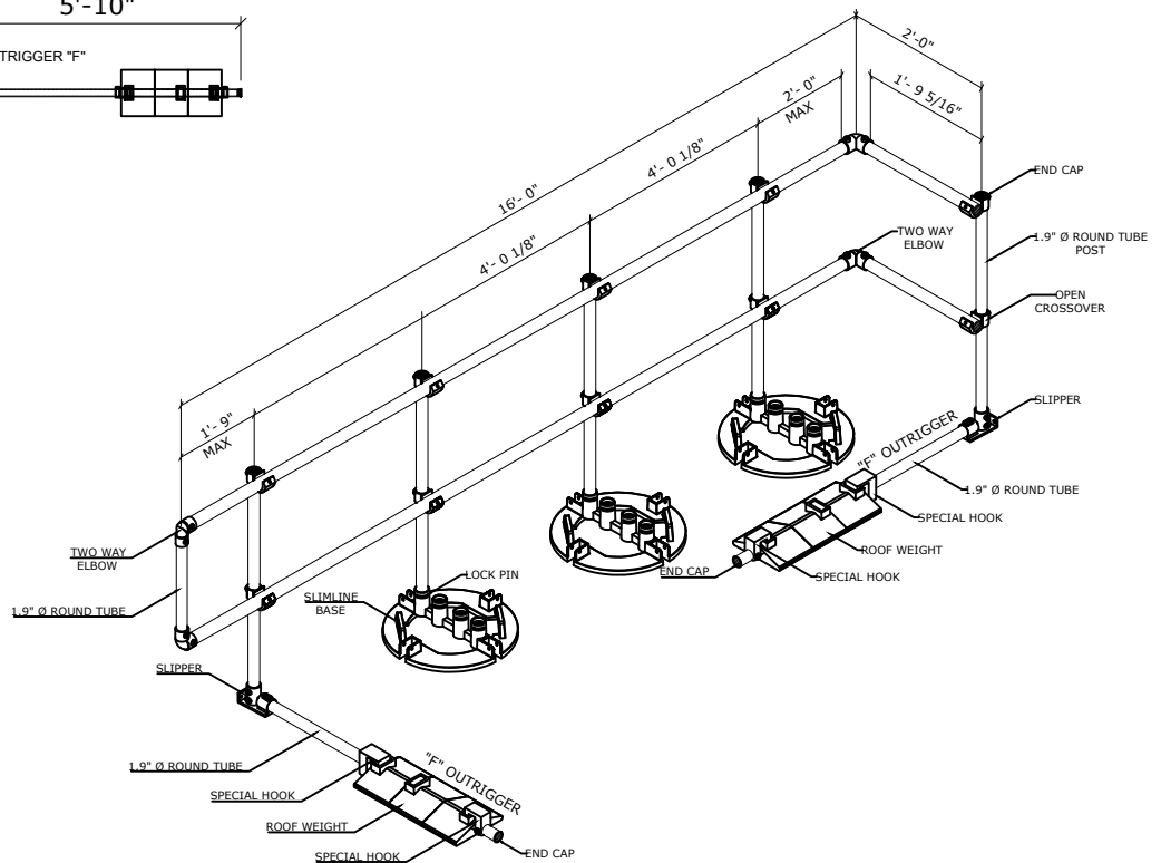
ISOMETRIC
