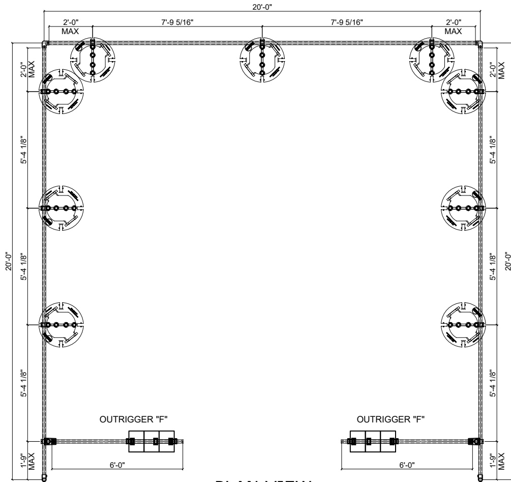
PLAN VIEW
