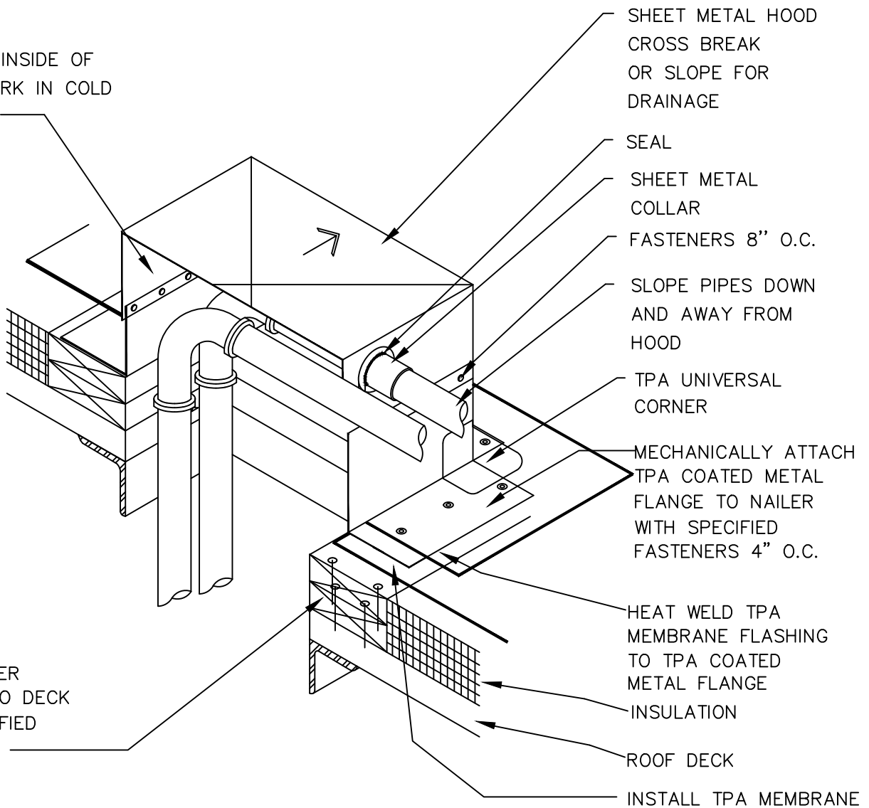
CLOSURE DETAIL
