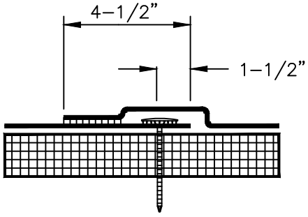
LAP CROSS SECTION
