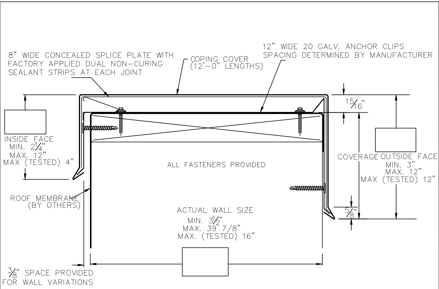
ANCHOR CLIP PROFILE ON WALLS GREATER THAT 14"
