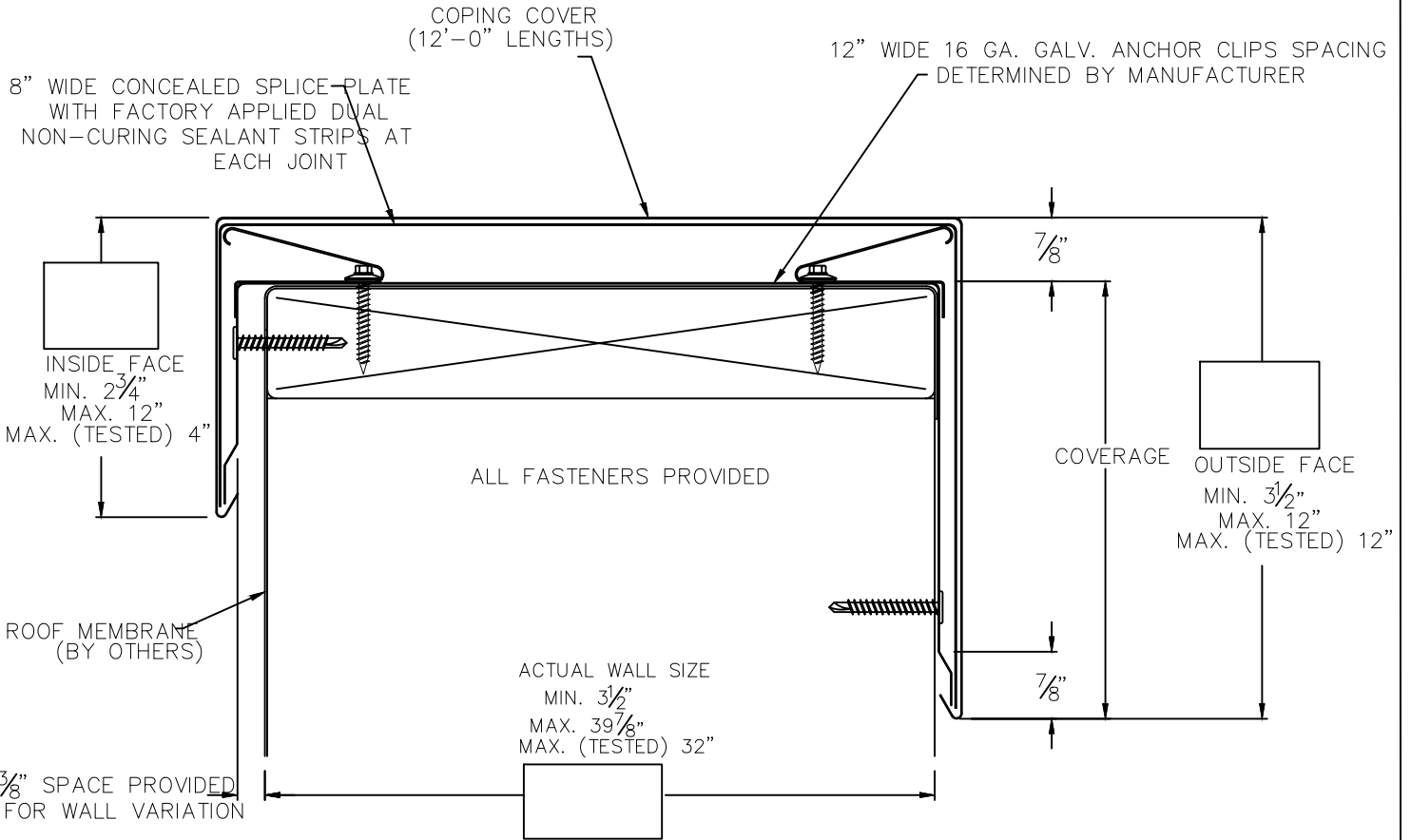
ANCHOR CLIP PROFILE ON WALLS GREATER THAN 14"
