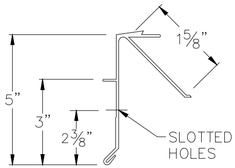
EXTRUDED PROFILE
