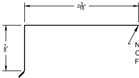
RAKE TRIM (ALTERNATIVE)
