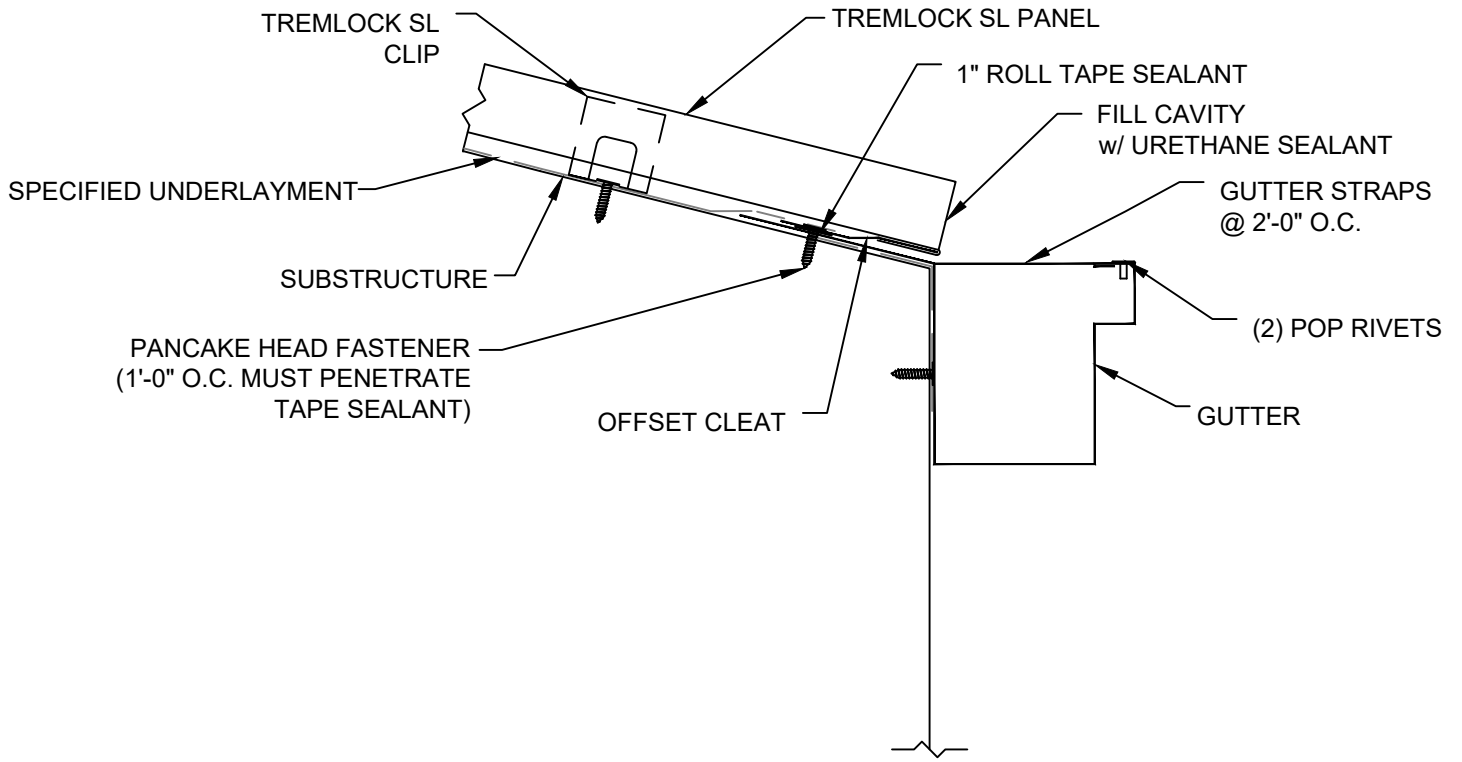
EAVE w/ STANDARD GUTTER
