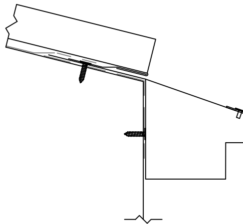
SUGGESTED FOR HIGH SNOW AREAS
