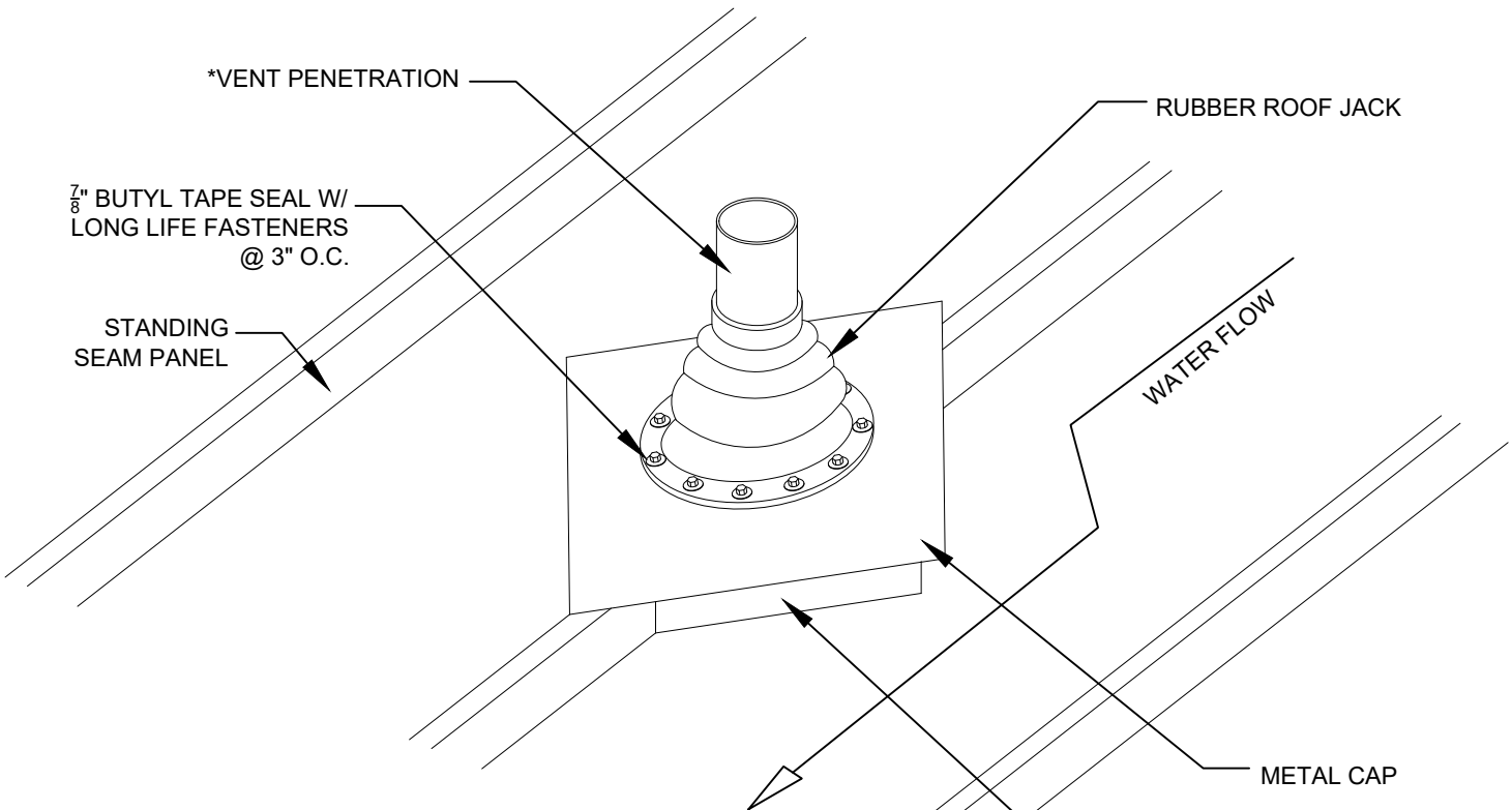
ALTERNATE PIPE DETAIL @ STANDING SEAM
