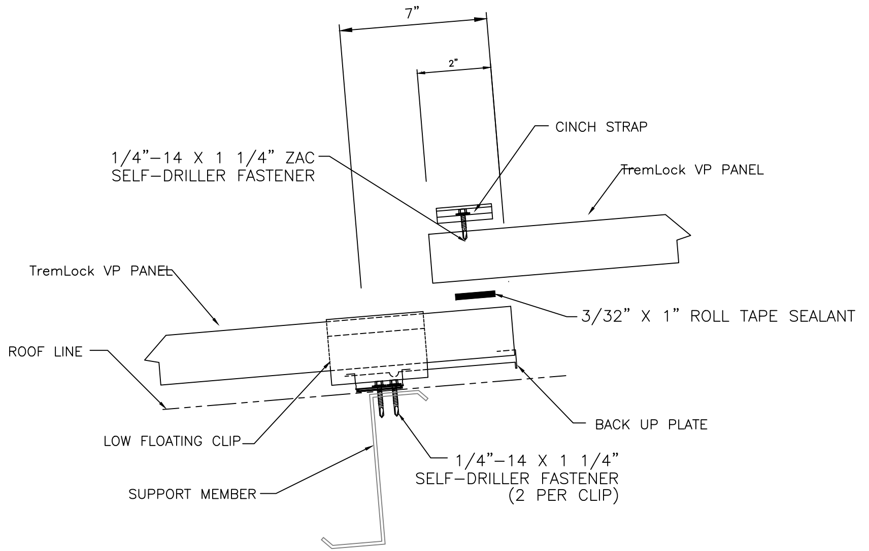
SECTION AT LAP/LOW FLOATING W/COMPRESSIBLE BLANKET INSULATION (NOT SHOWN)
