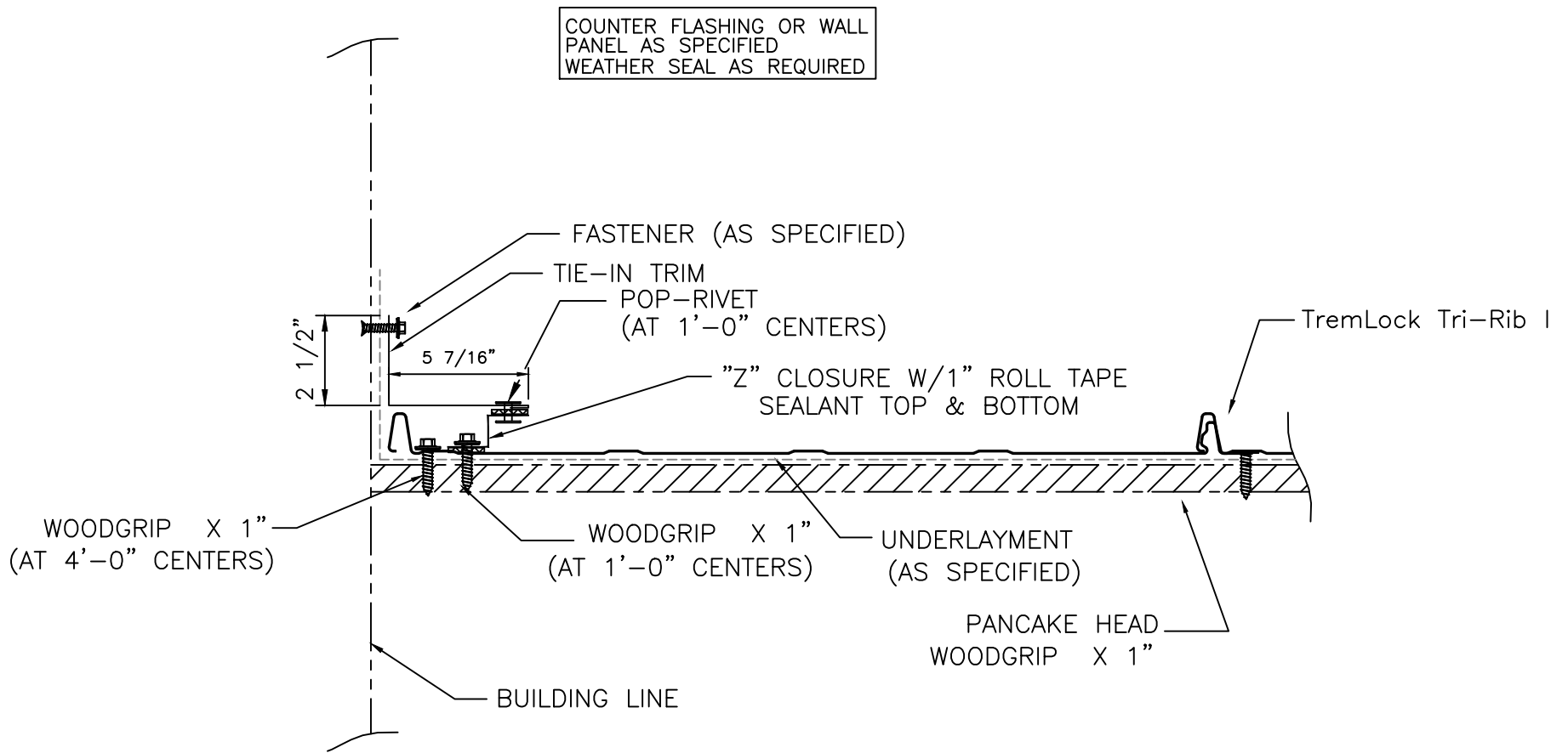
RAKE TIE-IN TRIM DETAIL (ARCHITECTURAL)
