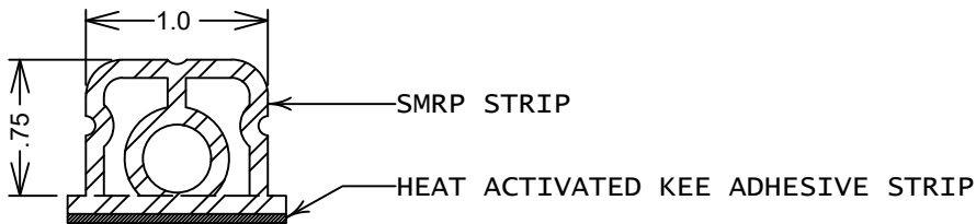
SMRP SECTION VIEW
