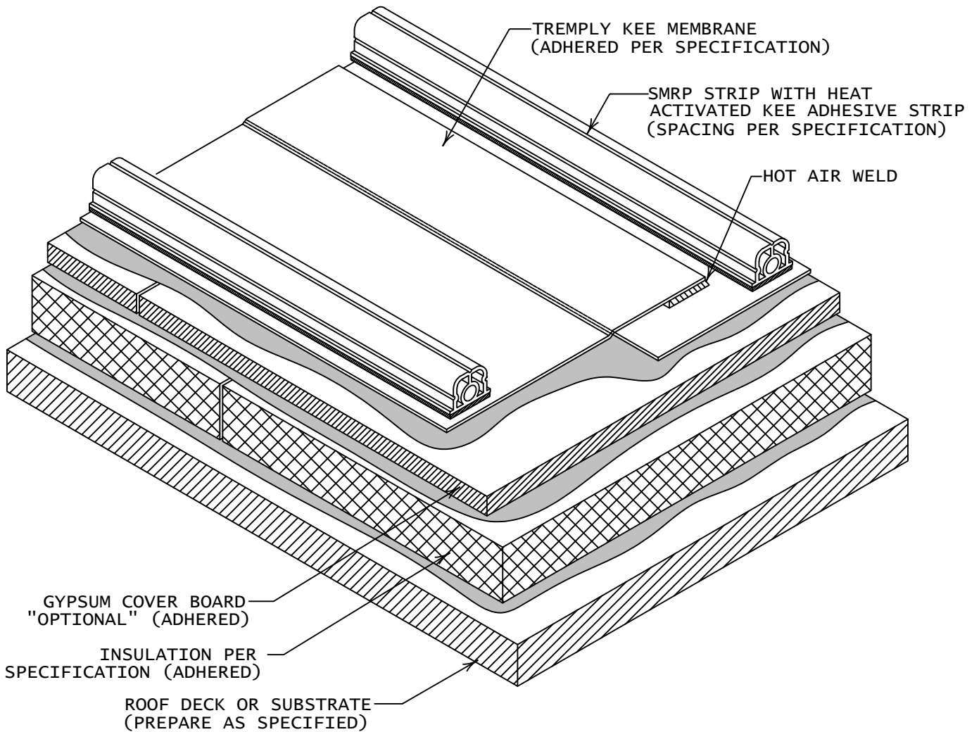
SMRP SECTION VIEW
