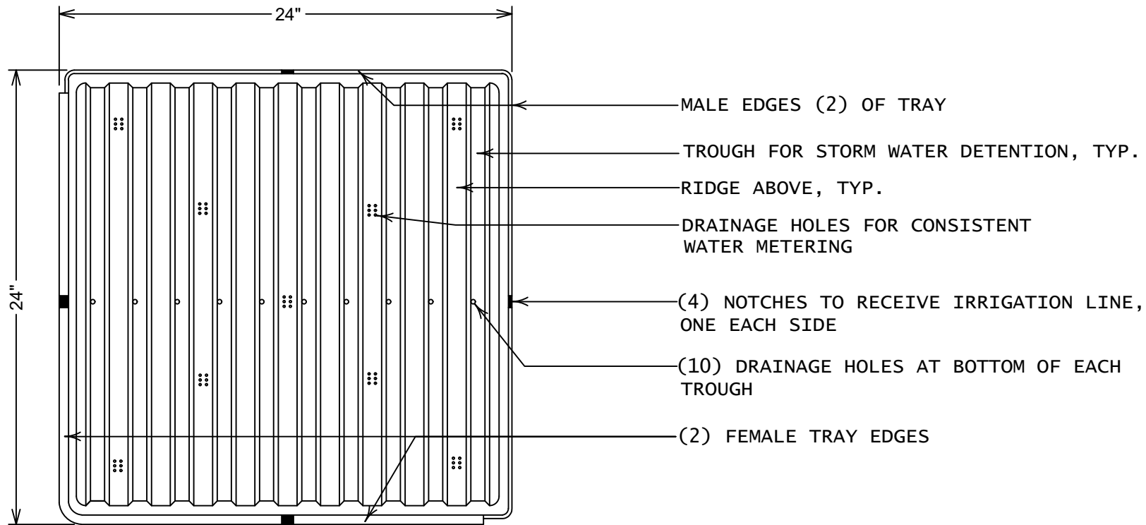
PLAN VIEW
