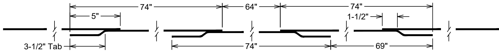
PANEL CONSTRUCTION
