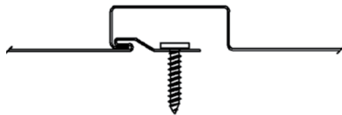
NOSTALGIA BOARD and BATTEN SEAM
