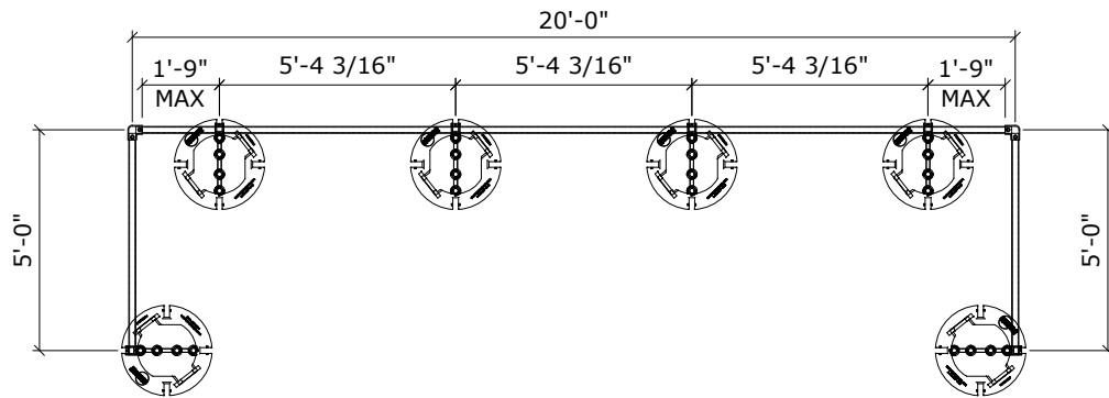
PLAN VIEW
